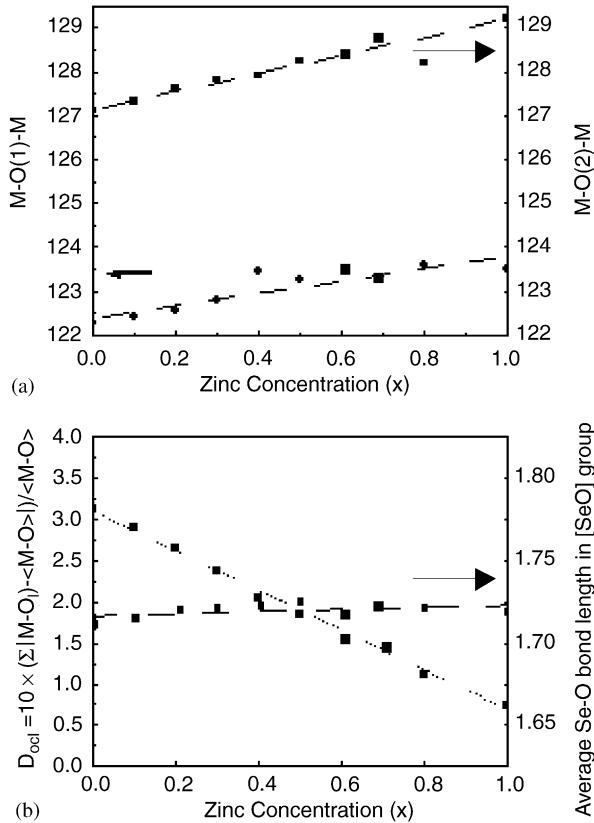
FIG. 5. (a) \langle M\text{-O}(1)\text{-}M \rangle and \langle M\text{-O}(2)\text{-}M \rangle bond angles vs zinc concentration (b) \text{MO}_6 octahedron distortion and average Se-O bond length in the [\text{SeO}]^{2-} group vs zinc concentration ( x ).
