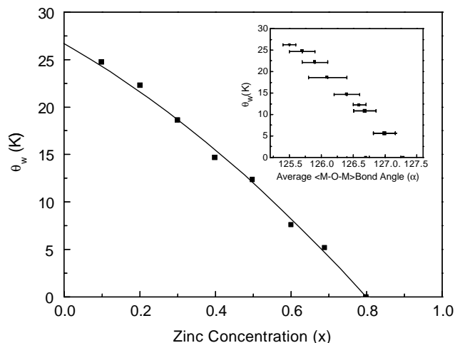
FIG. 7. Weiss constant ( \theta_w ) vs zinc concentration ( x ). The inset shows the Weiss constant ( \theta_w ) vs average \langle M-O-M \rangle bond angle plot.
